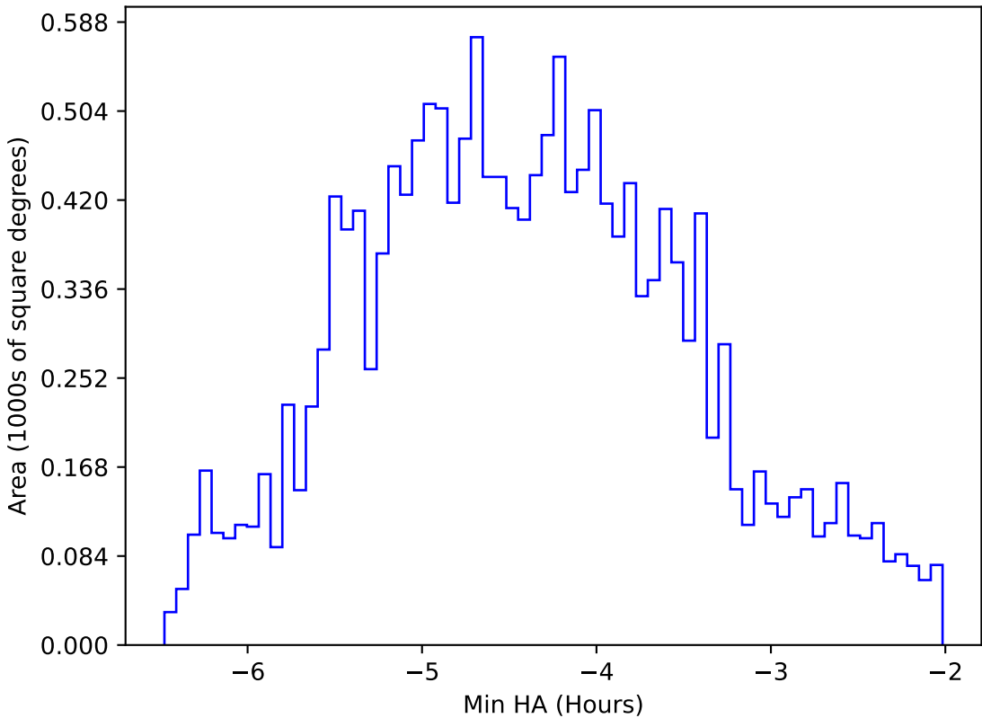
too_elab_heavy_r128_d2_ugrizy_v3.4_10yrs WFD z band: Min HA
