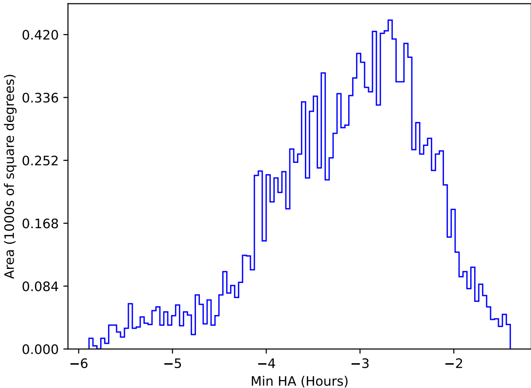
too_elab_heavy_r128_d2_ugrizy_v3.4_10yrs WFD u band: Min HA
