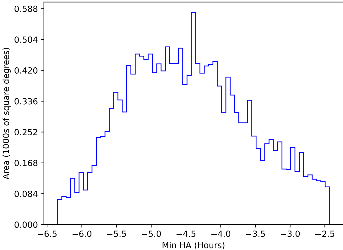
too_elab_heavy_r128_d2_ugrizy_v3.4_10yrs WFD r band: Min HA
