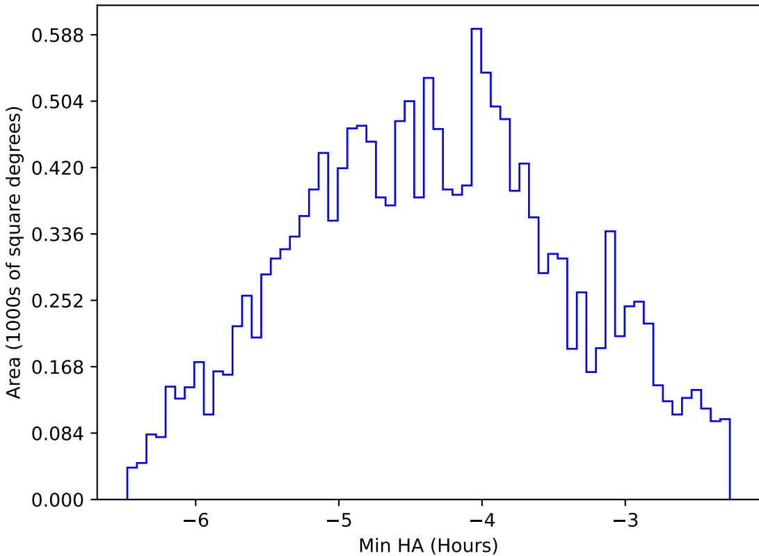
too_elab_heavy_r128_d2_ugrizy_v3.4_10yrs WFD i band: Min HA
