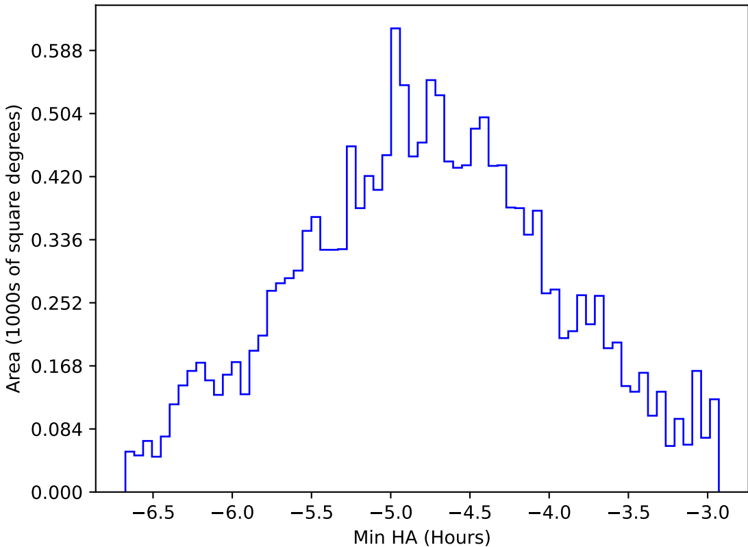
too_elab_heavy_r128_d2_ugrizy_v3.4_10yrs WFD all bands: Min HA
