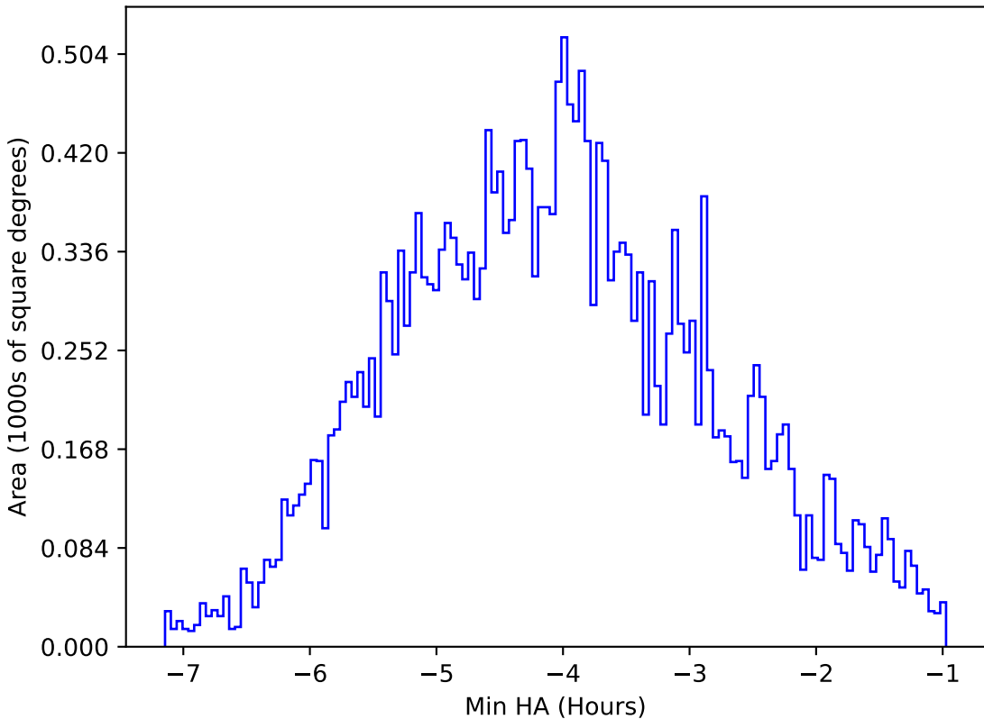
too_elab_heavy_r128_d2_ugrizy_v3.4_10yrs All sky i band: Min HA
