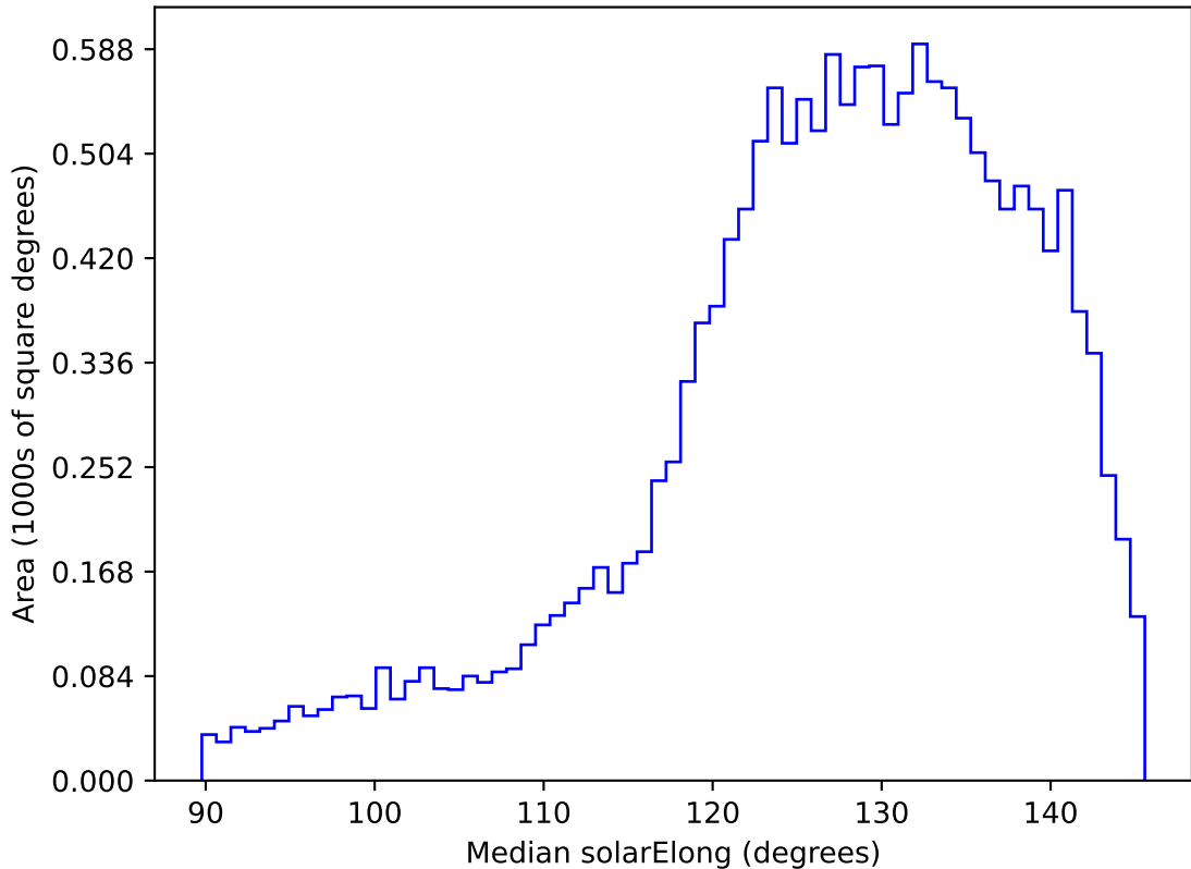
too_elab_heavy_r128_d2_ugrizy_v3.4_10yrs WFD z band: Median solarElong
