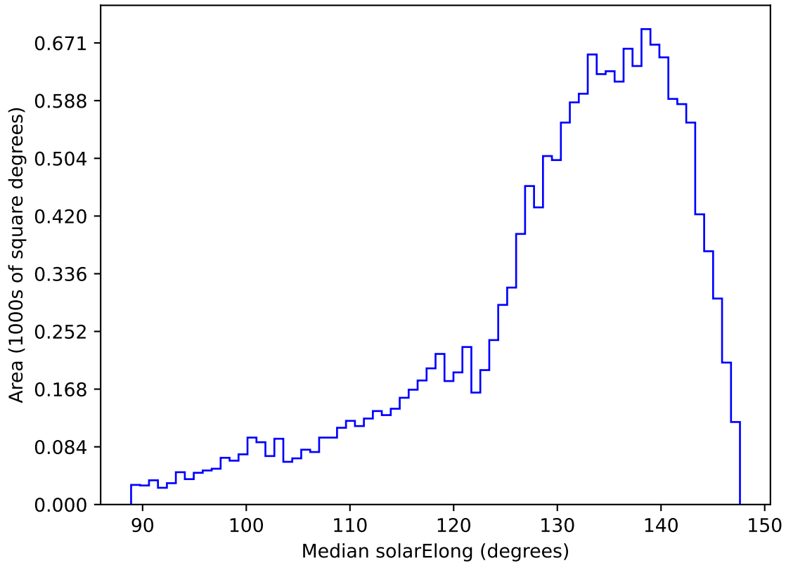
too_elab_heavy_r128_d2_ugrizy_v3.4_10yrs WFD y band: Median solarElong
