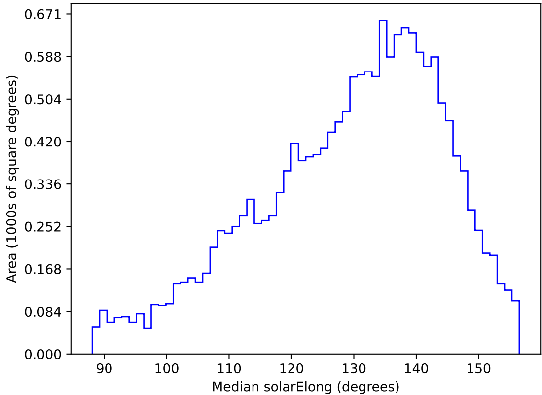
too_elab_heavy_r128_d2_ugrizy_v3.4_10yrs WFD g band: Median solarElong
