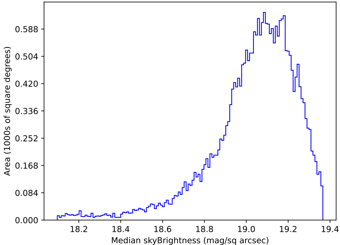
too_elab_heavy_r128_d2_ugrizy_v3.4_10yrs Yr 1 z band: Median skyBrightness
