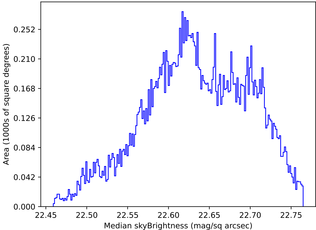
too_elab_heavy_r128_d2_ugrizy_v3.4_10yrs Yr 1 u band: Median skyBrightness
