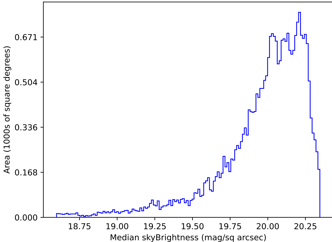
too_elab_heavy_r128_d2_ugrizy_v3.4_10yrs Yr 1 i band: Median skyBrightness
