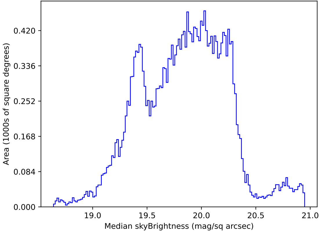
too_elab_heavy_r128_d2_ugrizy_v3.4_10yrs Yr 1 all bands: Median skyBrightness
