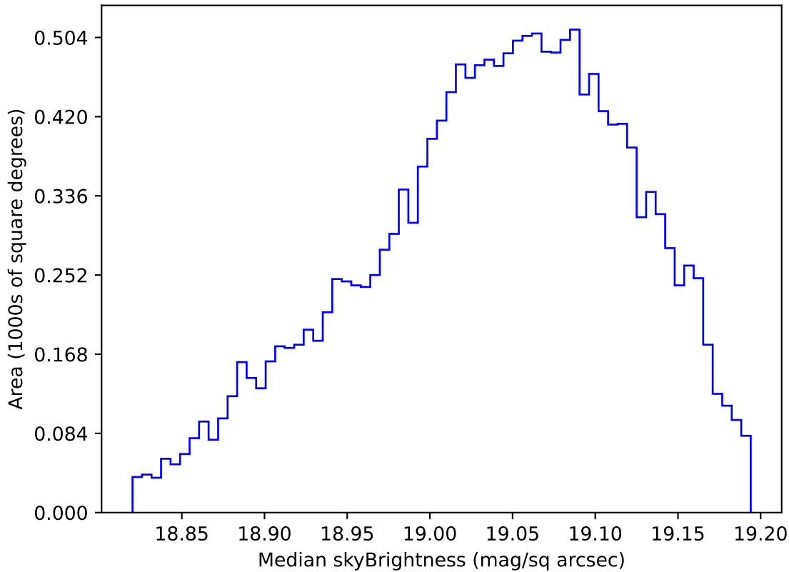
too_elab_heavy_r128_d2_ugrizy_v3.4_10yrs WFD z band: Median skyBrightness
