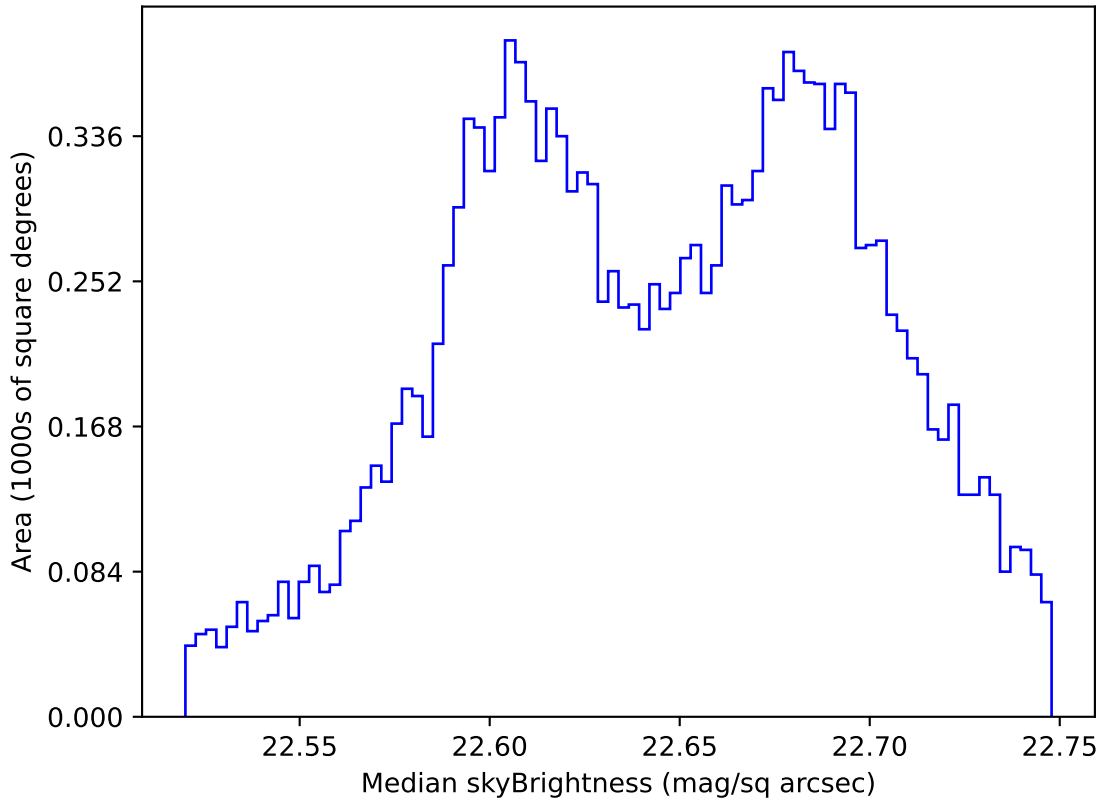
too_elab_heavy_r128_d2_ugrizy_v3.4_10yrs WFD u band: Median skyBrightness
