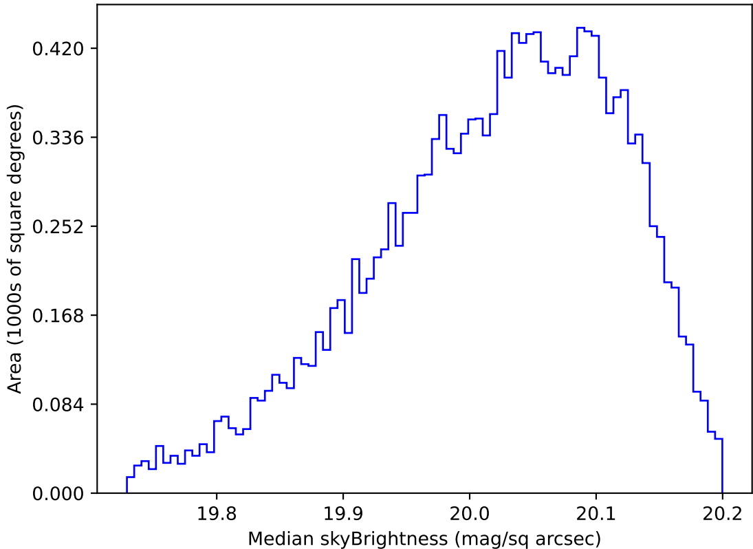
too_elab_heavy_r128_d2_ugrizy_v3.4_10yrs WFD i band: Median skyBrightness
