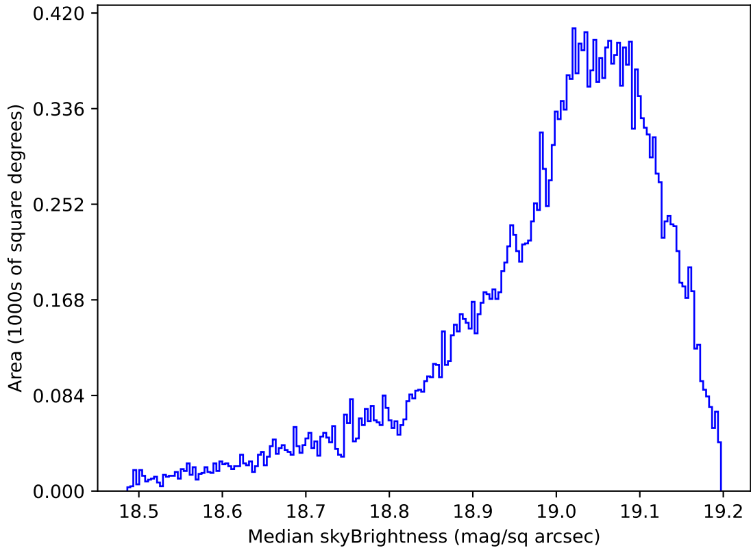
too_elab_heavy_r128_d2_ugrizy_v3.4_10yrs All sky z band: Median skyBrightness
