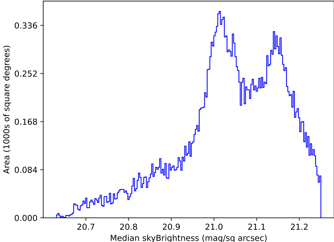
too_elab_heavy_r128_d2_ugrizy_v3.4_10yrs All sky r band: Median skyBrightness
