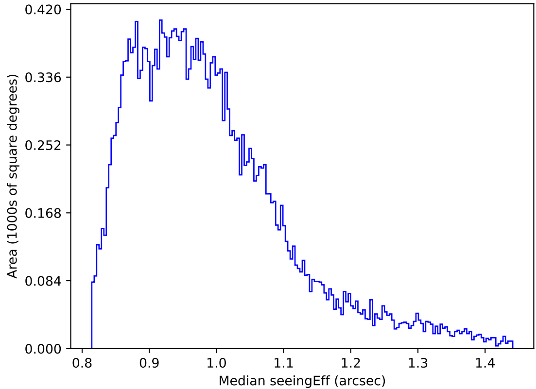
too_elab_heavy_r128_d2_ugrizy_v3.4_10yrs Yr 1 all bands: Median seeingEff
