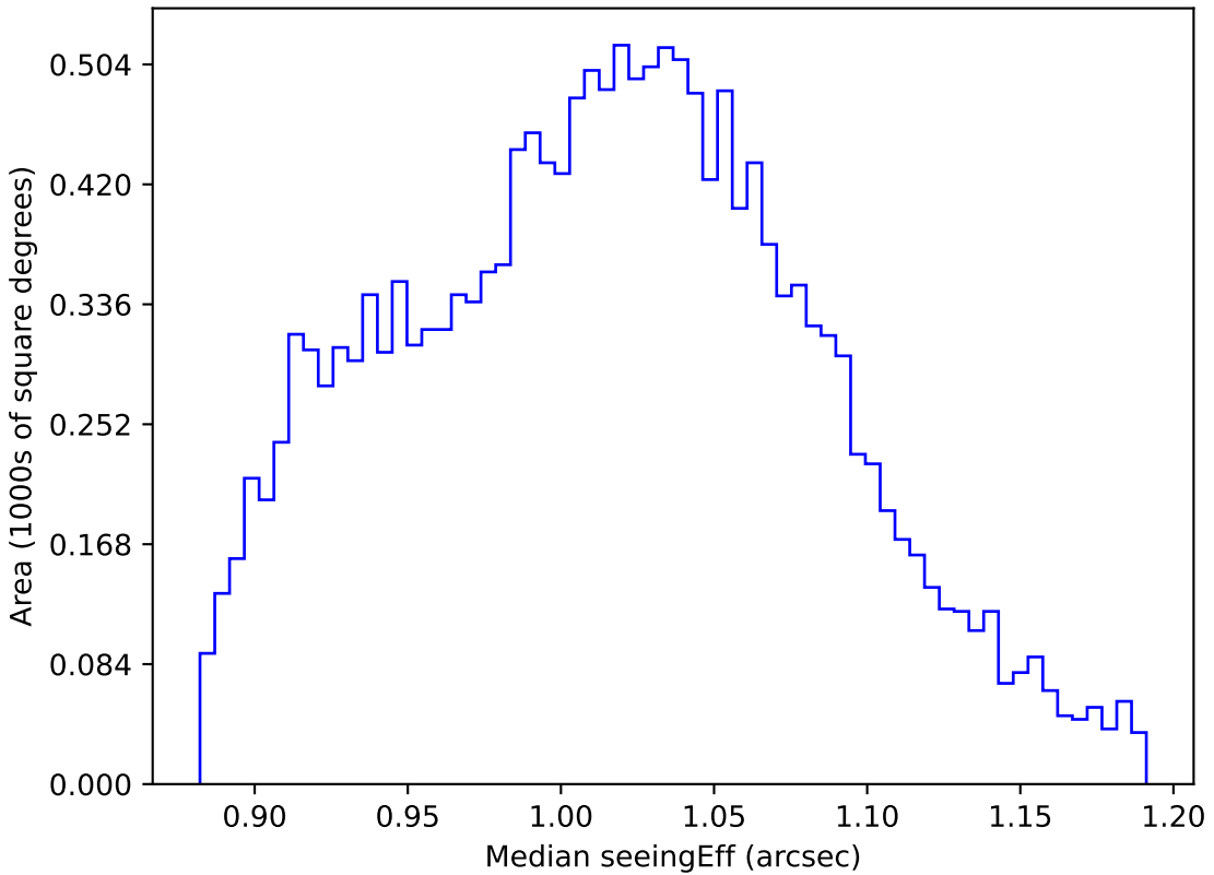
too_elab_heavy_r128_d2_ugrizy_v3.4_10yrs WFD z band: Median seeingEff
