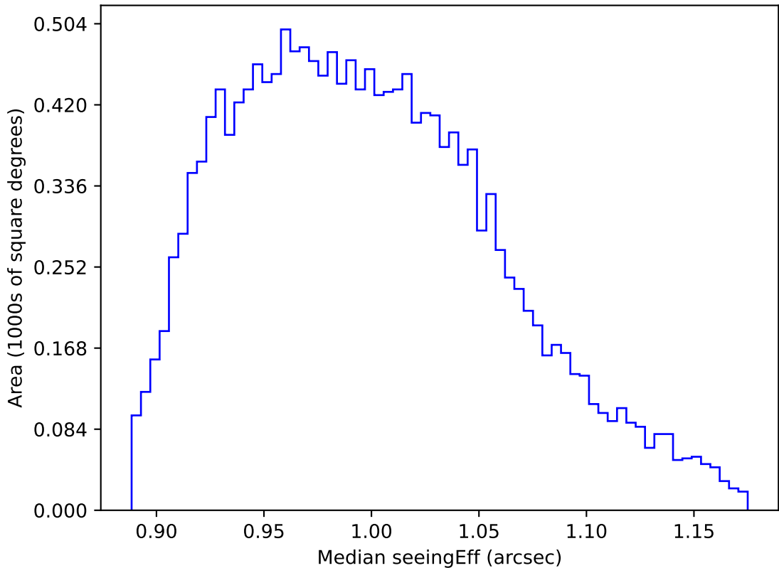
too_elab_heavy_r128_d2_ugrizy_v3.4_10yrs WFD y band: Median seeingEff
