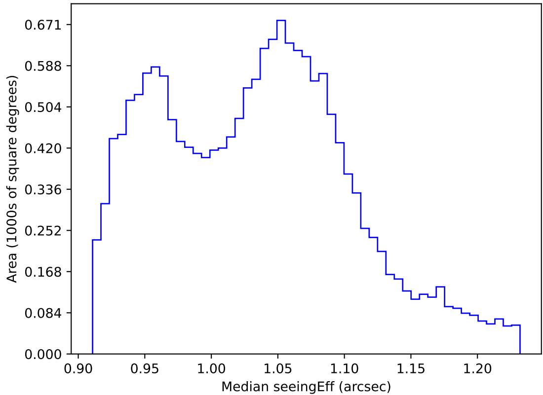
too_elab_heavy_r128_d2_ugrizy_v3.4_10yrs WFD all bands: Median seeingEff
