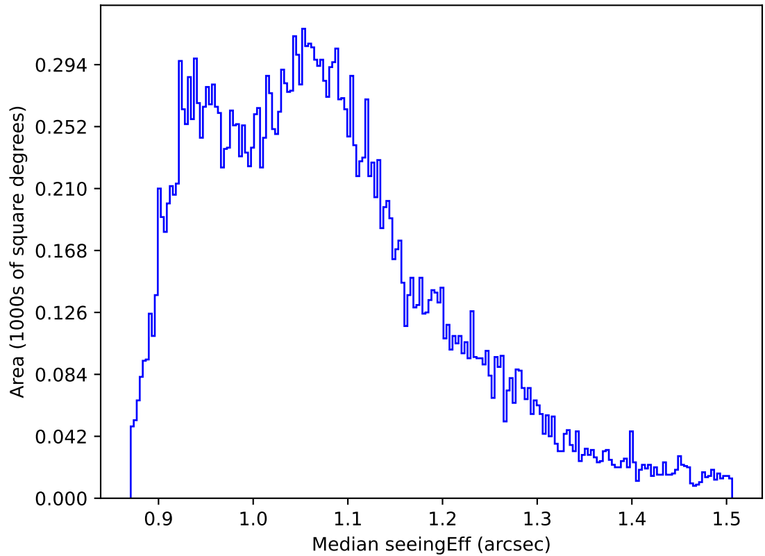
too_elab_heavy_r128_d2_ugrizy_v3.4_10yrs All sky r band: Median seeingEff
