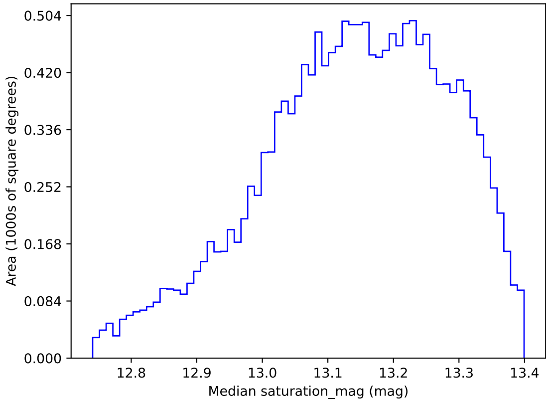
too_elab_heavy_r128_d2_ugrizy_v3.4_10yrs WFD y band: Median saturation_mag
