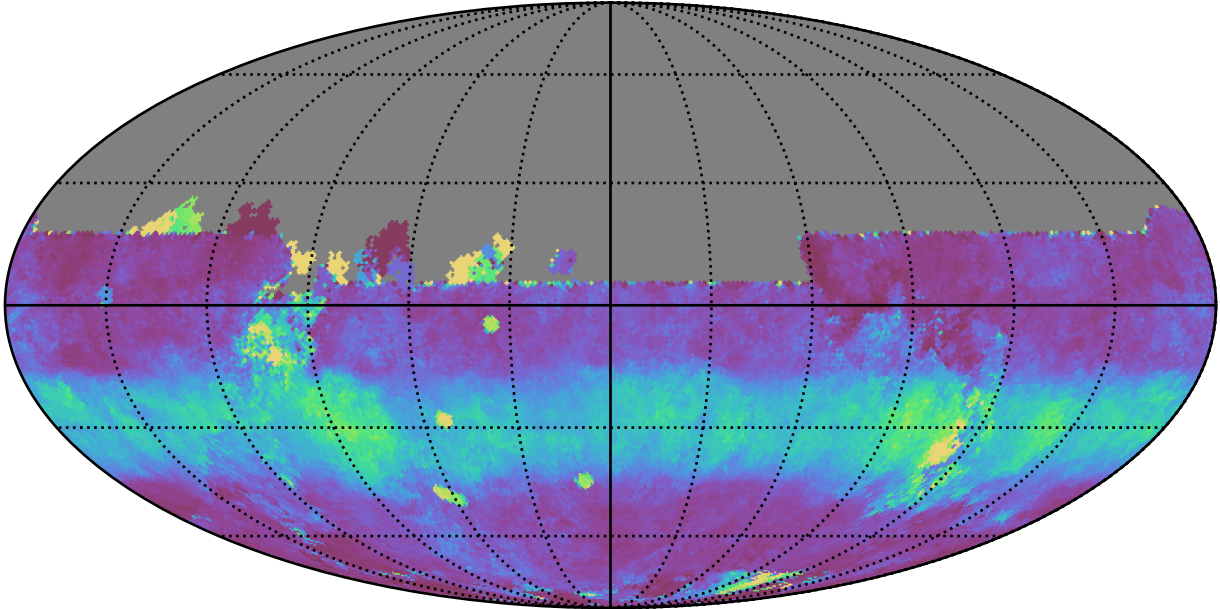
too_elab_heavy_r128_d2_ugrizy_v3.4_10yrs All sky y band: Median normairmass
