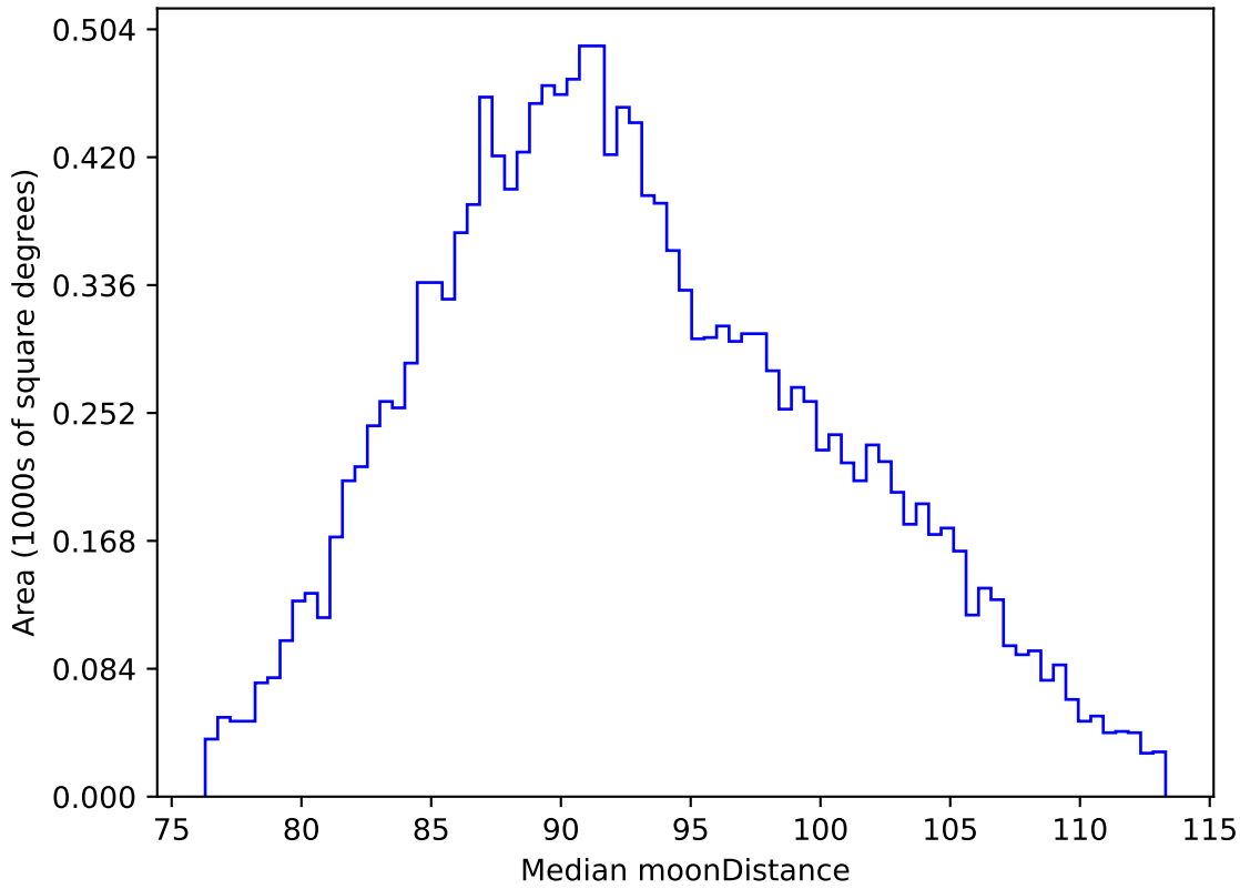
too_elab_heavy_r128_d2_ugrizy_v3.4_10yrs WFD i band: Median moonDistance
