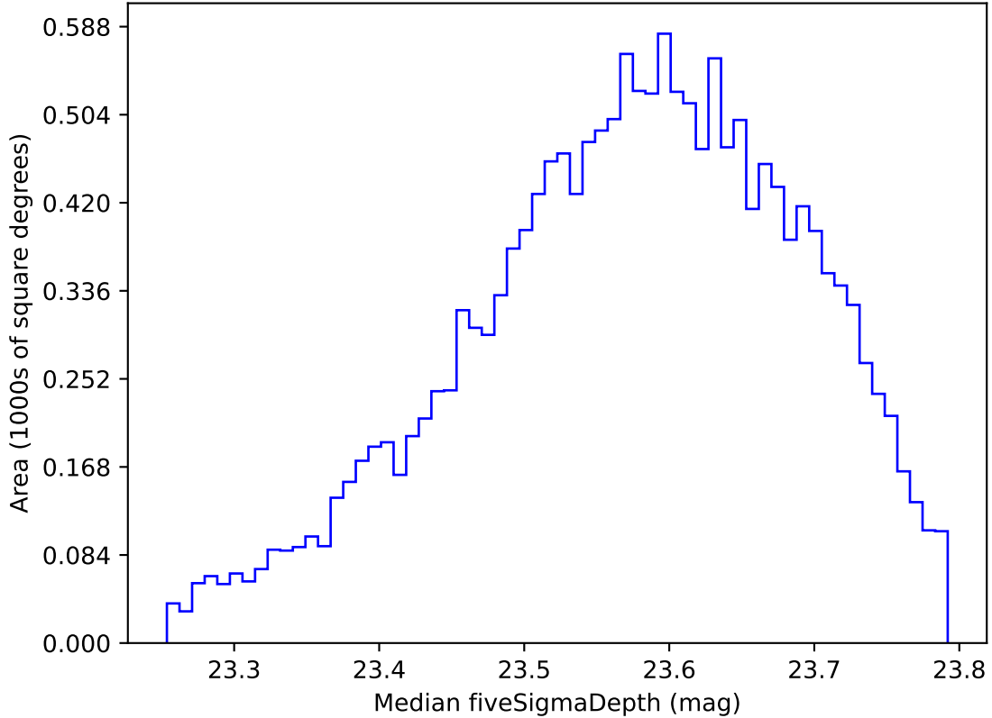
too_elab_heavy_r128_d2_ugrizy_v3.4_10yrs WFD i band: Median fiveSigmaDepth
