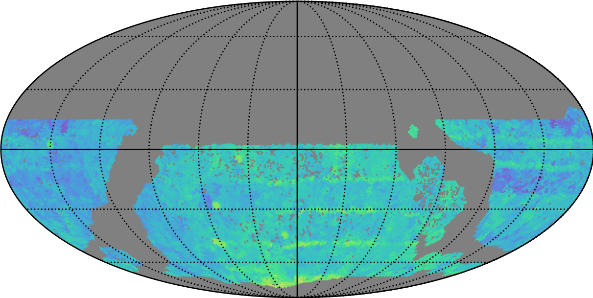
too_elab_heavy_r128_d2_ugrizy_v3.4_10yrs WFD z band: Median Season Length
