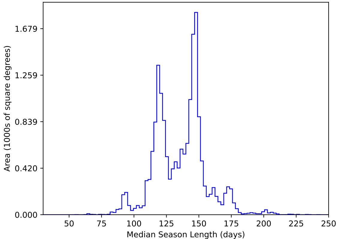
too_elab_heavy_r128_d2_ugrizy_v3.4_10yrs WFD y band: Median Season Length
