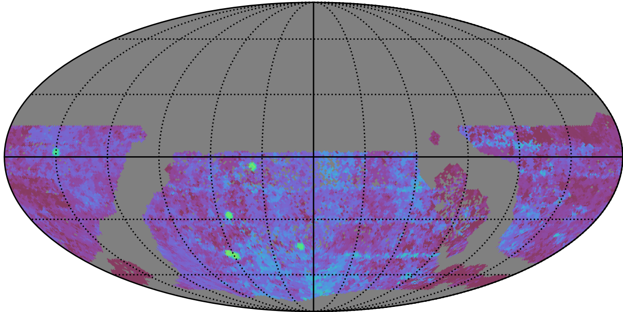
too_elab_heavy_r128_d2_ugrizy_v3.4_10yrs WFD u band: Median Season Length
