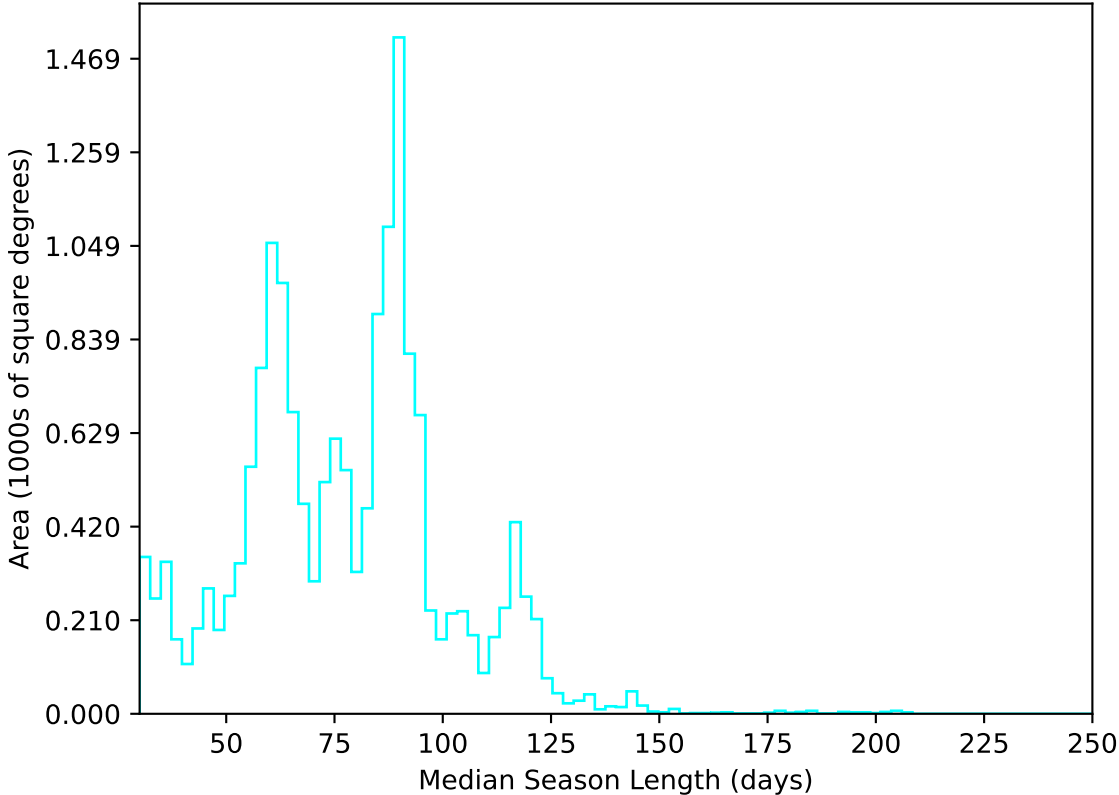
too_elab_heavy_r128_d2_ugrizy_v3.4_10yrs WFD u band: Median Season Length
