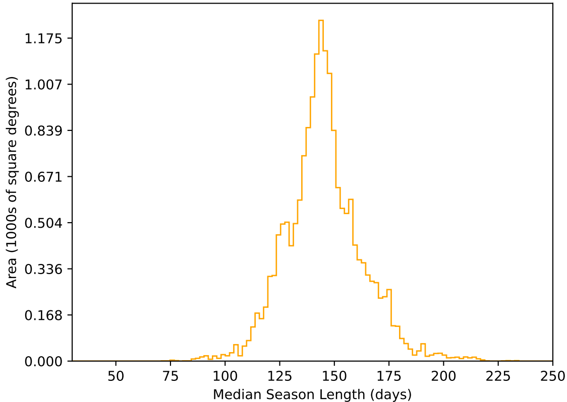
too_elab_heavy_r128_d2_ugrizy_v3.4_10yrs WFD r band: Median Season Length
