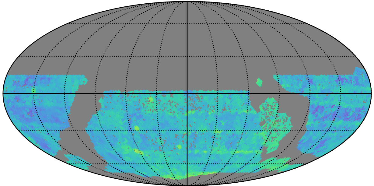
too_elab_heavy_r128_d2_ugrizy_v3.4_10yrs WFD i band: Median Season Length
