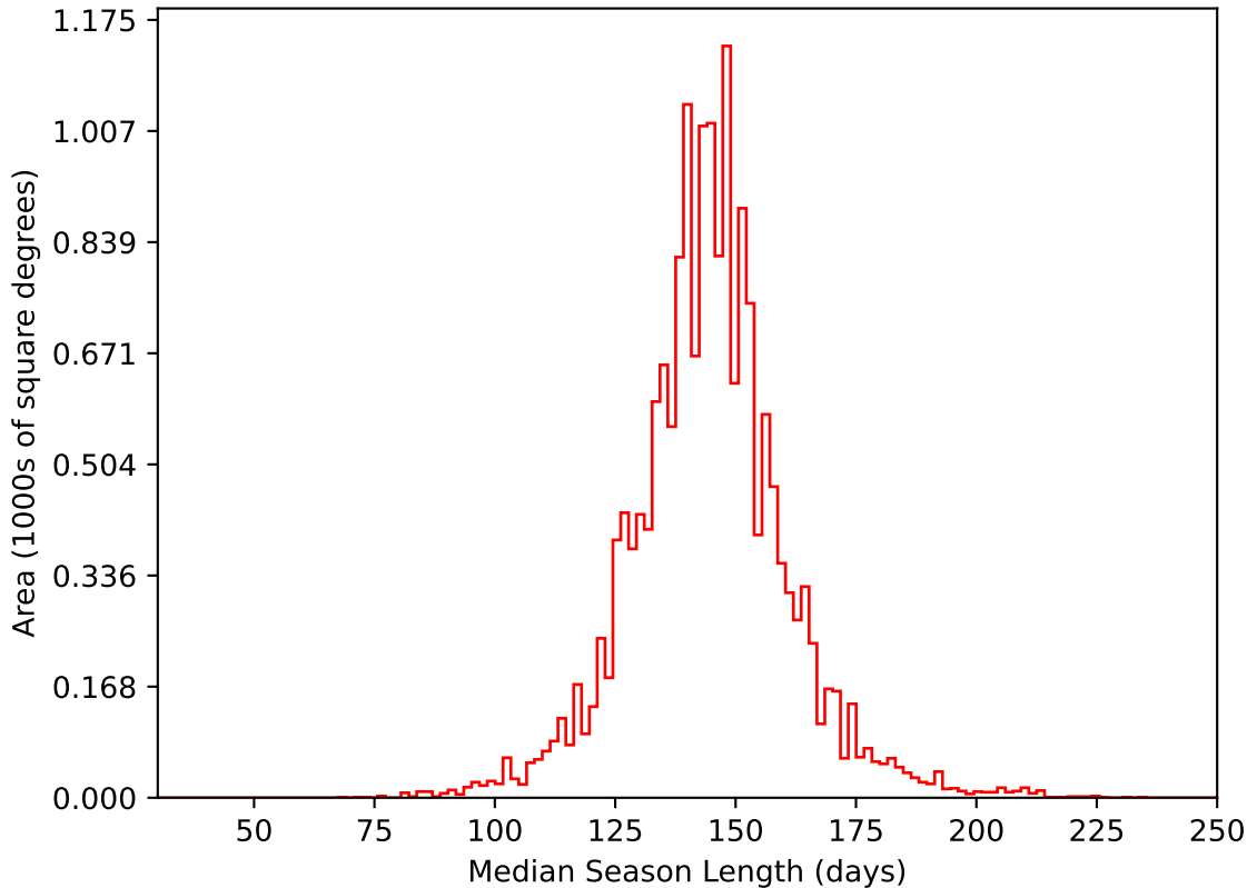
too_elab_heavy_r128_d2_ugrizy_v3.4_10yrs WFD i band: Median Season Length
