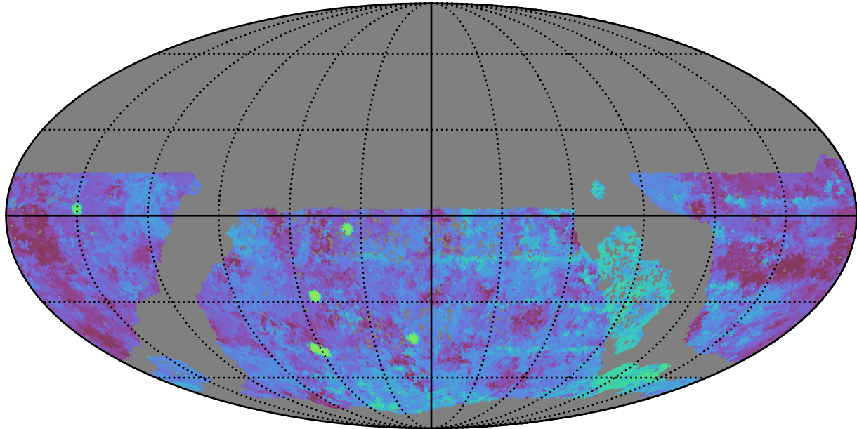
too_elab_heavy_r128_d2_ugrizy_v3.4_10yrs WFD g band: Median Season Length
