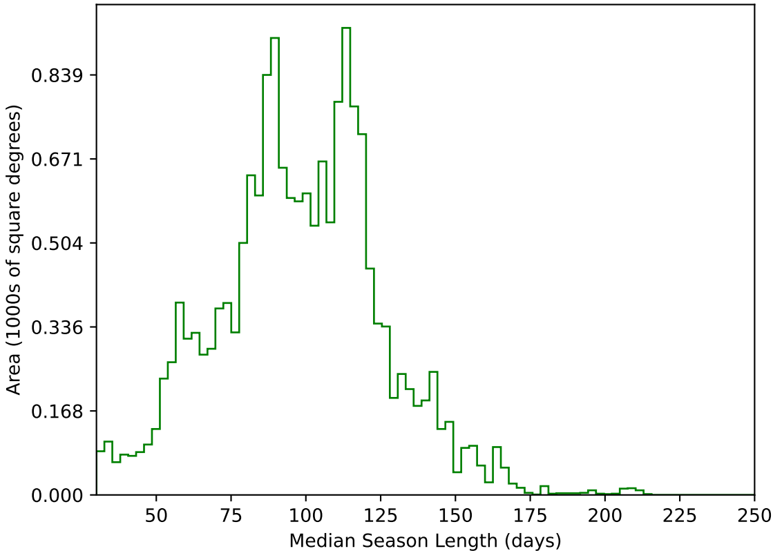
too_elab_heavy_r128_d2_ugrizy_v3.4_10yrs WFD g band: Median Season Length
