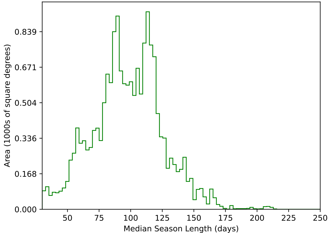
too_elab_heavy_r128_d2_ugrizy_v3.4_10yrs WFD g band: Median Season Length
