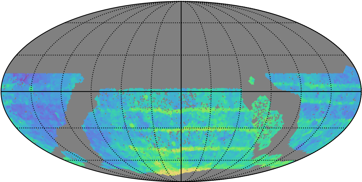
too_elab_heavy_r128_d2_ugrizy_v3.4_10yrs WFD all bands: Median Season Length
