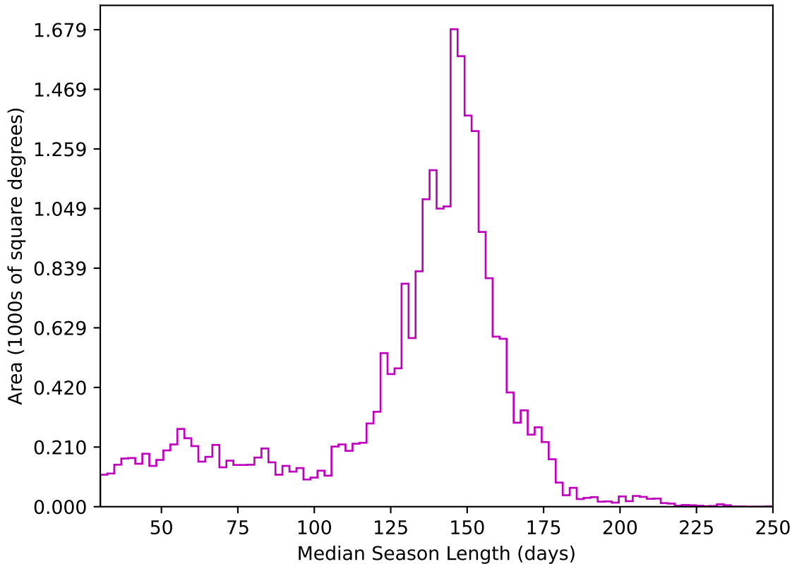
too_elab_heavy_r128_d2_ugrizy_v3.4_10yrs All sky z band: Median Season Length
