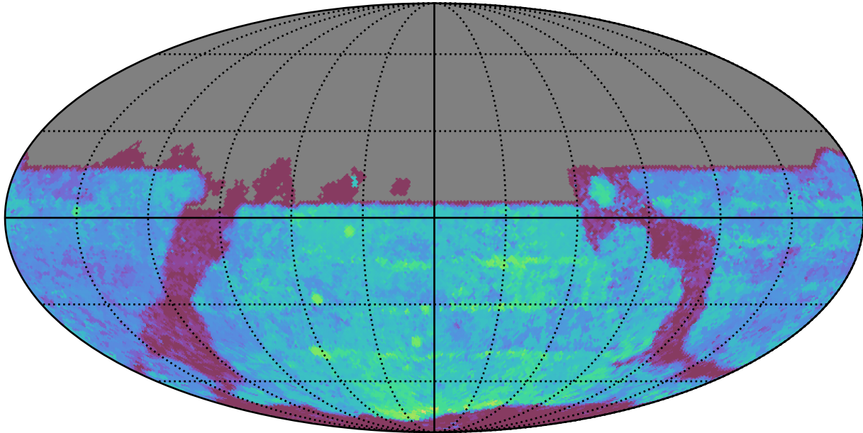
too_elab_heavy_r128_d2_ugrizy_v3.4_10yrs All sky y band: Median Season Length
