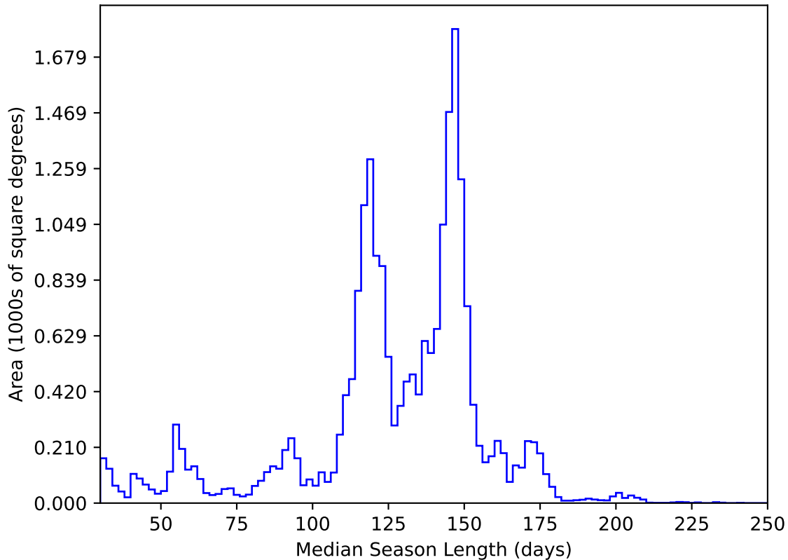
too_elab_heavy_r128_d2_ugrizy_v3.4_10yrs All sky y band: Median Season Length
