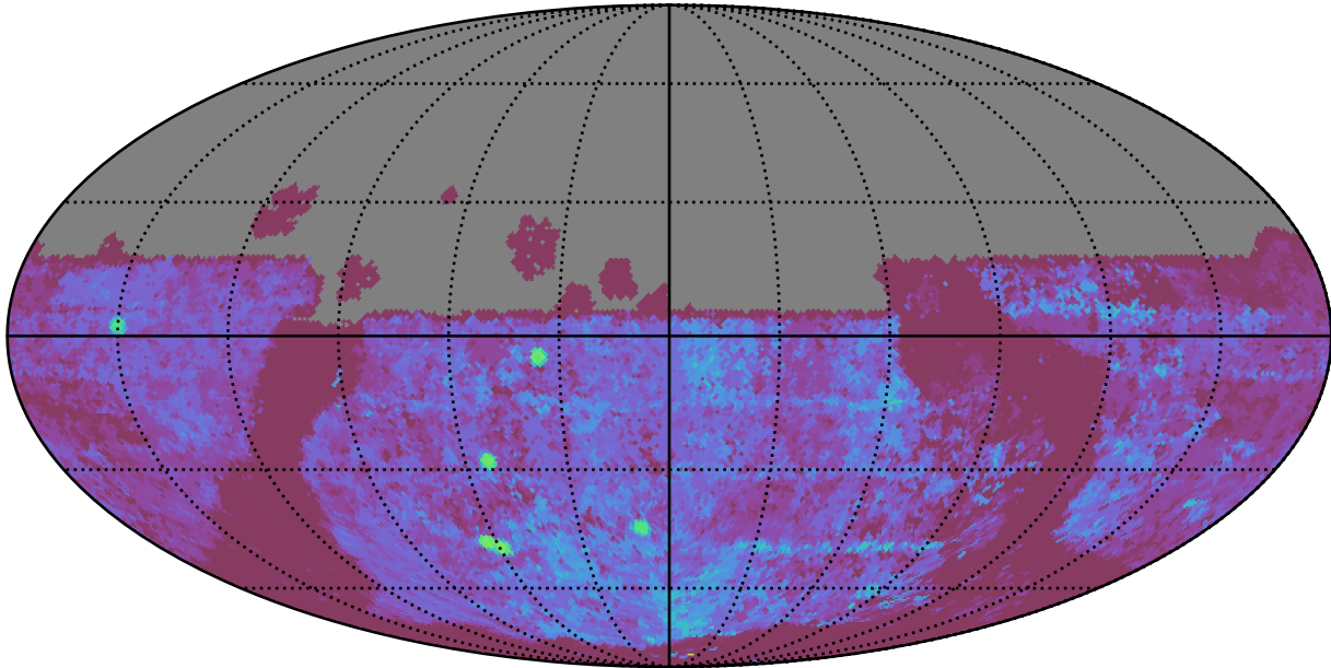
too_elab_heavy_r128_d2_ugrizy_v3.4_10yrs All sky u band: Median Season Length
