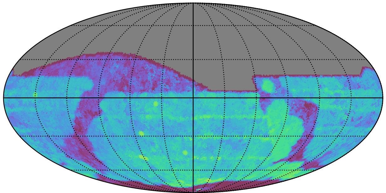
too_elab_heavy_r128_d2_ugrizy_v3.4_10yrs All sky r band: Median Season Length
