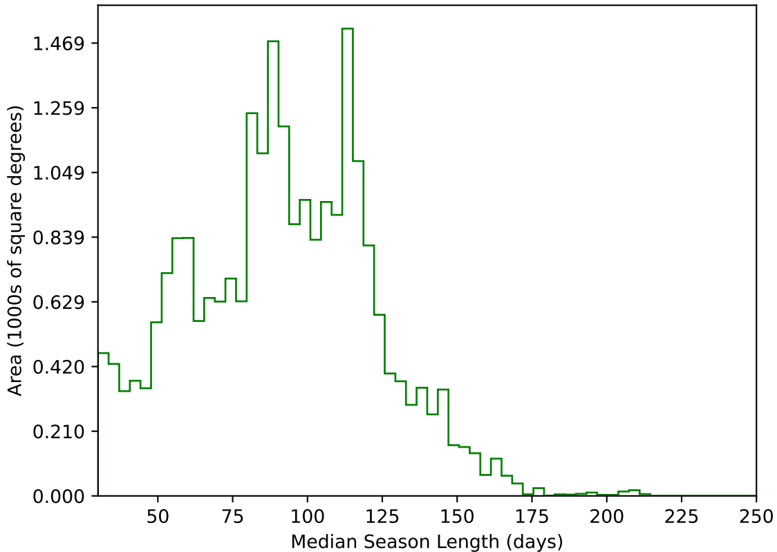
too_elab_heavy_r128_d2_ugrizy_v3.4_10yrs All sky g band: Median Season Length
