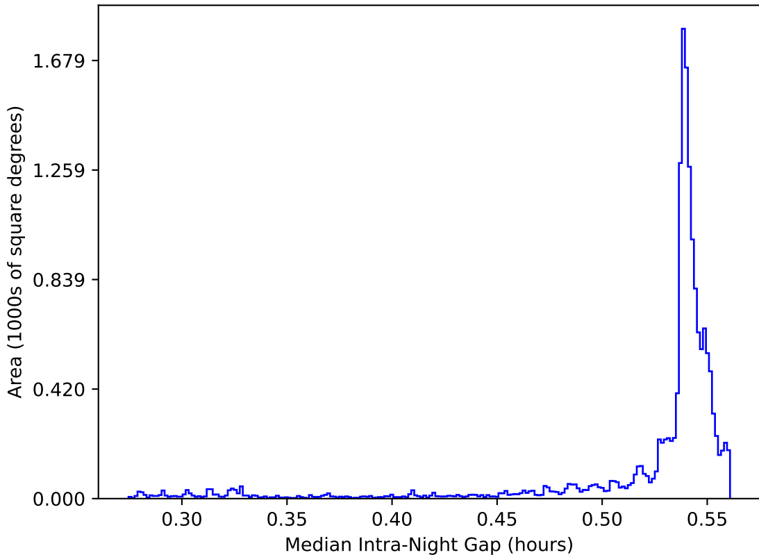
too_elab_heavy_r128_d2_ugrizy_v3.4_10yrs WFD: Median Intra-Night Gap
