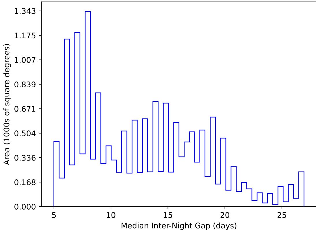
too_elab_heavy_r128_d2_ugrizy_v3.4_10yrs WFD y band: Median Inter-Night Gap
