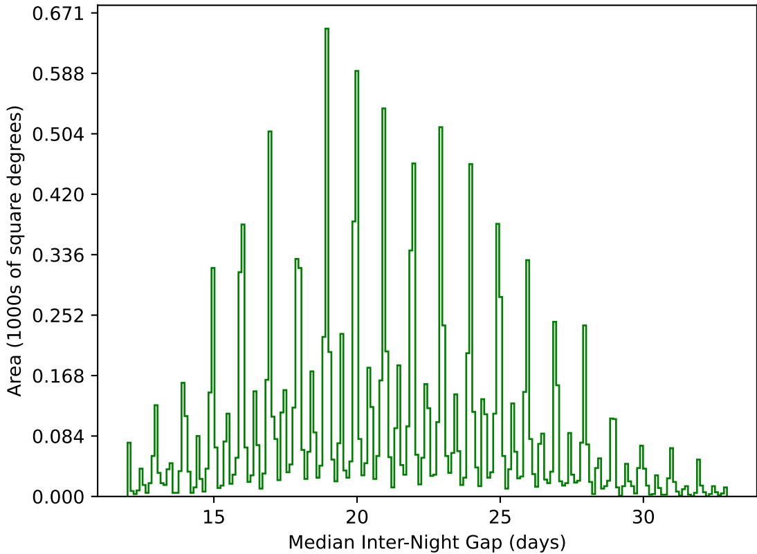
too_elab_heavy_r128_d2_ugrizy_v3.4_10yrs WFD g band: Median Inter-Night Gap
