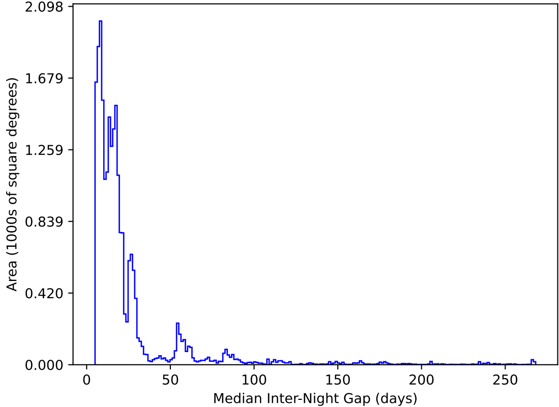
too_elab_heavy_r128_d2_ugrizy_v3.4_10yrs All sky y band: Median Inter-Night Gap
