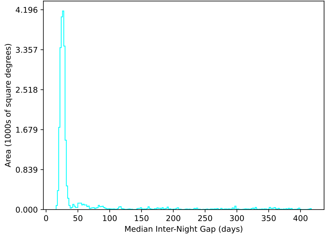
too_elab_heavy_r128_d2_ugrizy_v3.4_10yrs All sky u band: Median Inter-Night Gap
