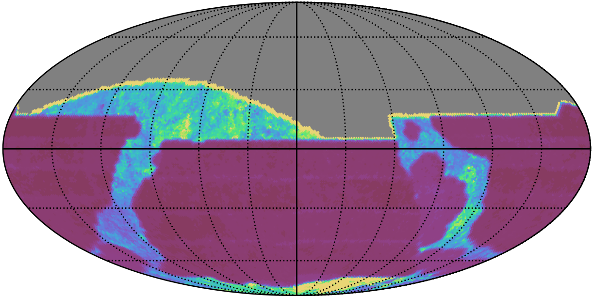
too_elab_heavy_r128_d2_ugrizy_v3.4_10yrs All sky all bands: Median Inter-Night Gap
