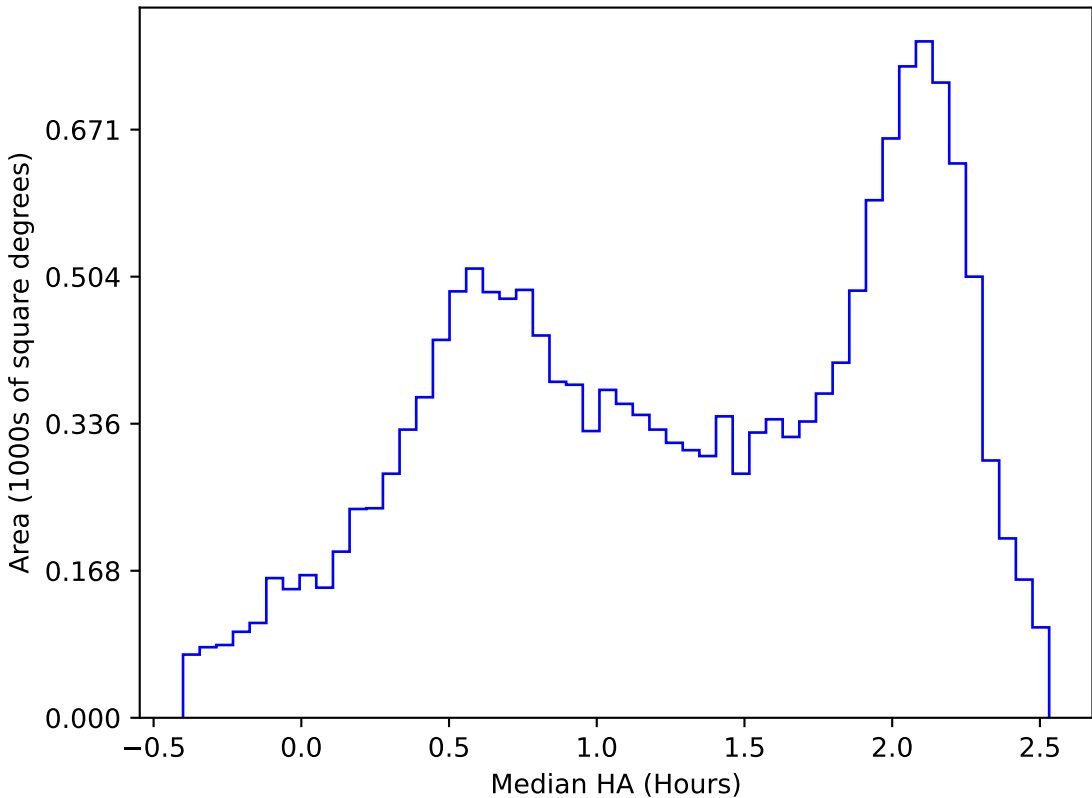
too_elab_heavy_r128_d2_ugrizy_v3.4_10yrs WFD y band: Median HA
